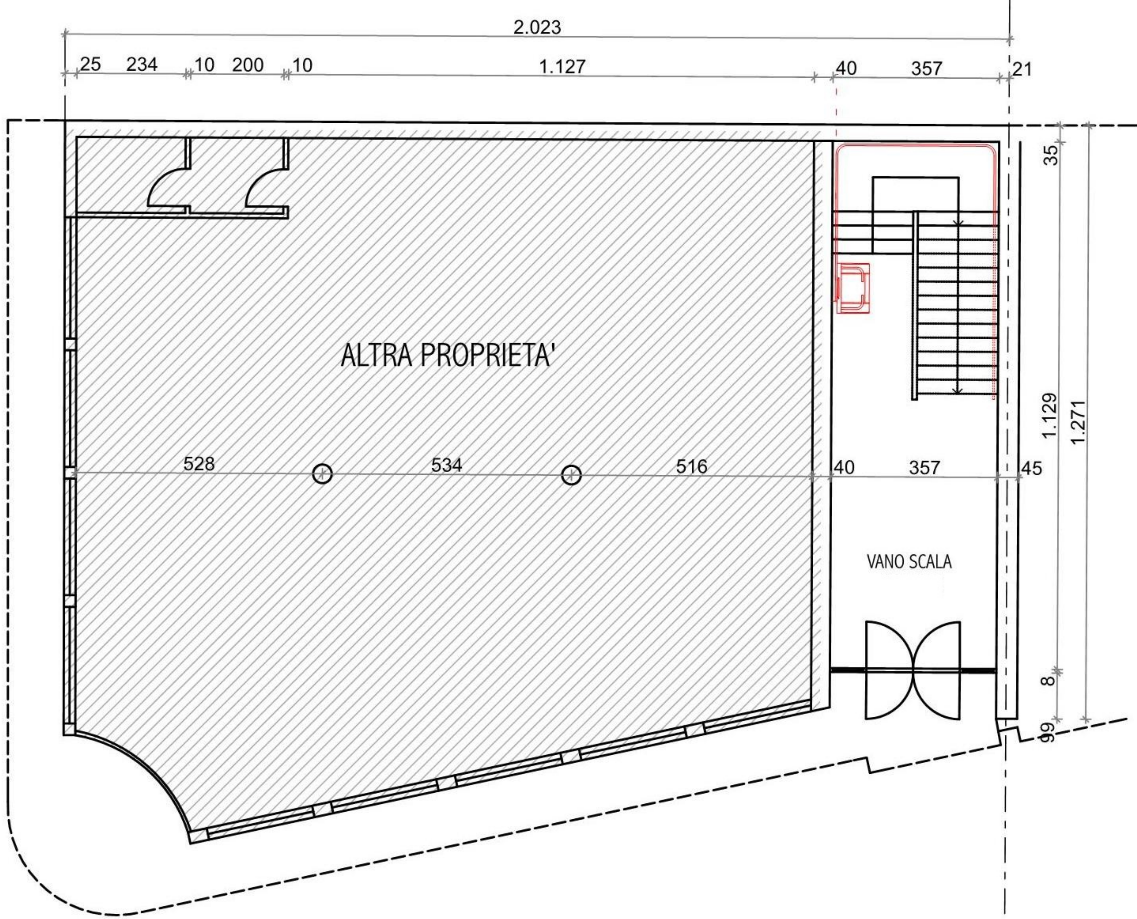
PIANO TERRA
